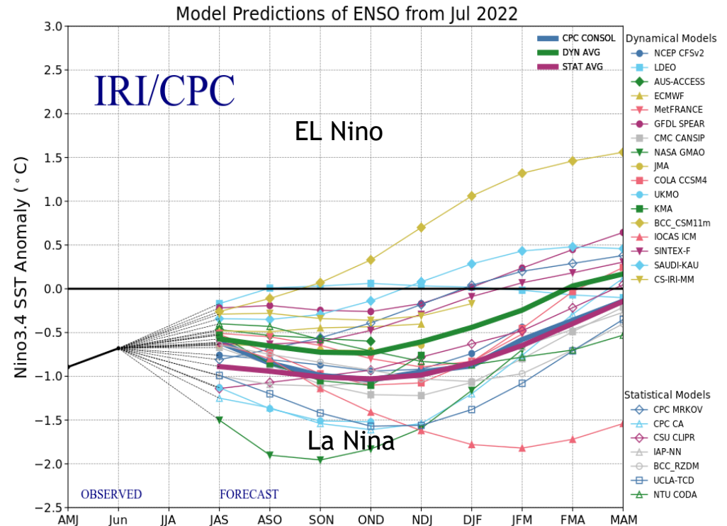
Figure provided by the International Research Institute (IRI) for Climate and Society (updated 19 July 2022).
